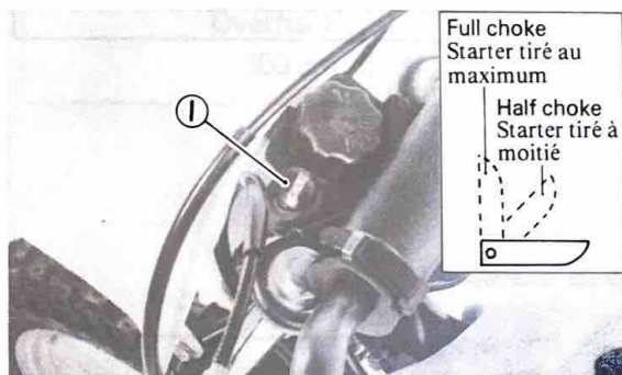
1. Starter lever 1. Levier de starter
