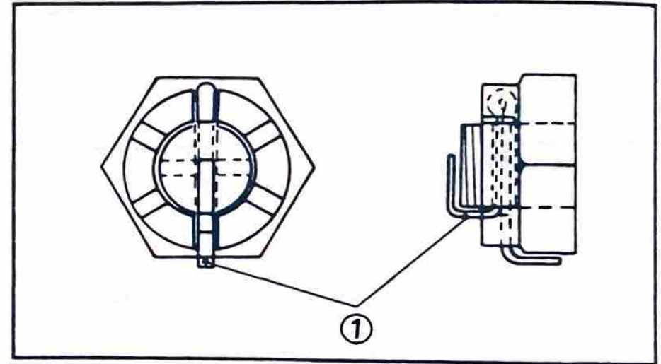
1. Cotter pin
