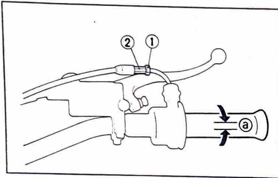
1. Lock nut 2. Adjuster a. 3~5 mm (0.12~0.20 in)
