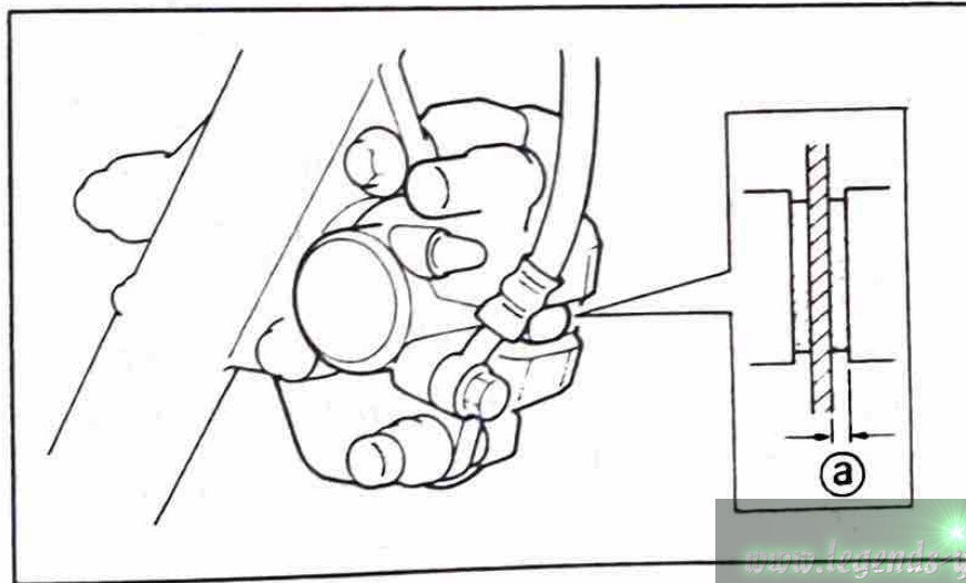
a. Wear limit 0.8 mm (0.031 in)
