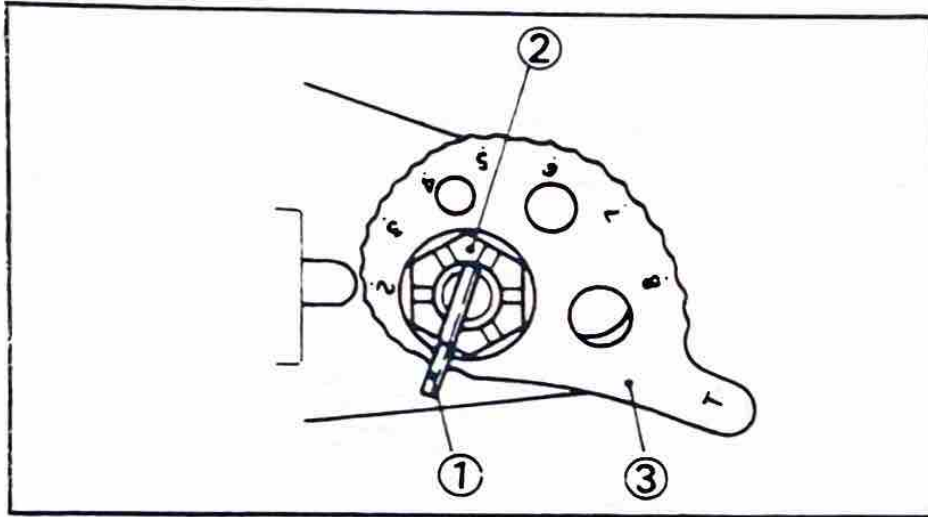
1. Cotter pin 2. Axle nut 3. Chain puller
