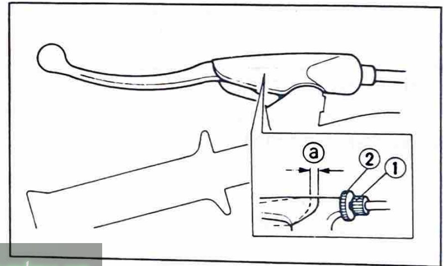
1. Adjuster 2. Lock nut a. 2~3 mm (0.08~0.12 in)
