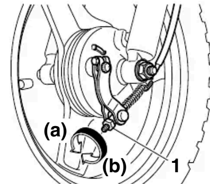
1. Brake lever free play adjusting nut
