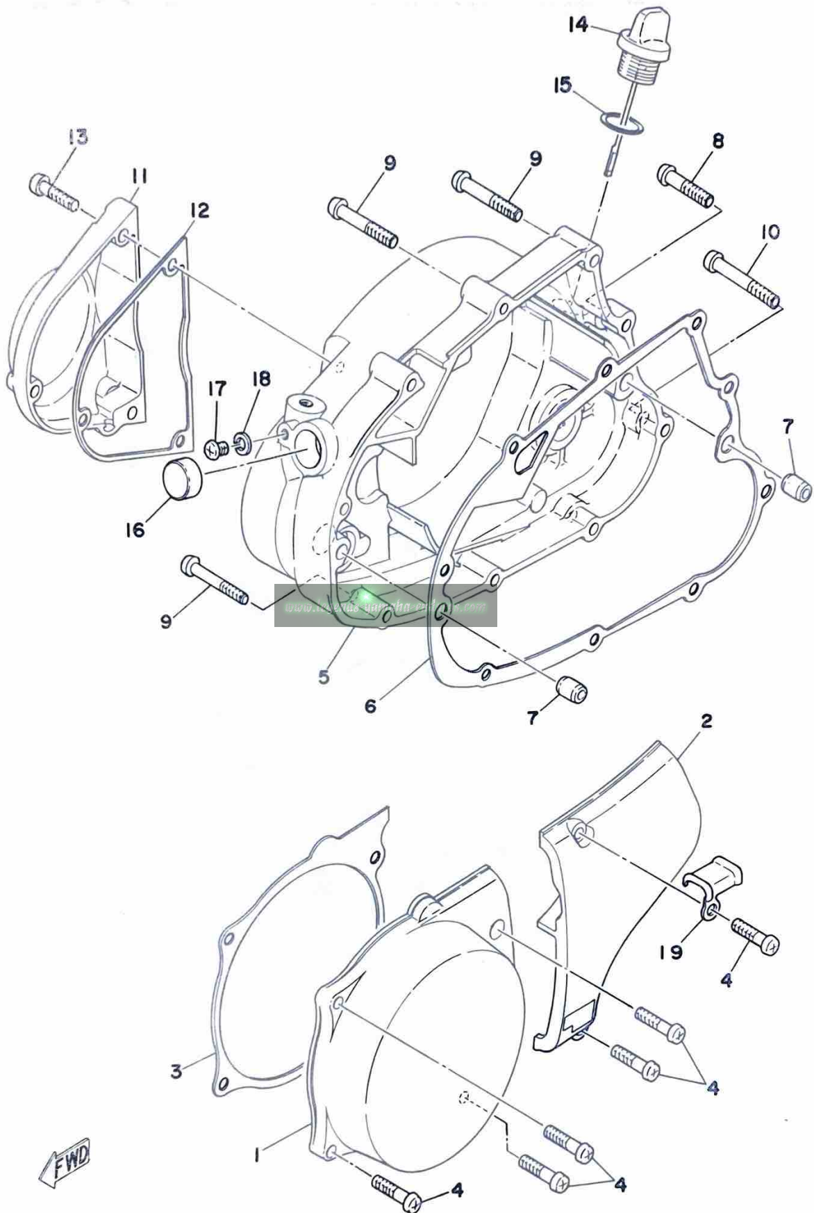
Fig. 2 CRANKCASE COVER
