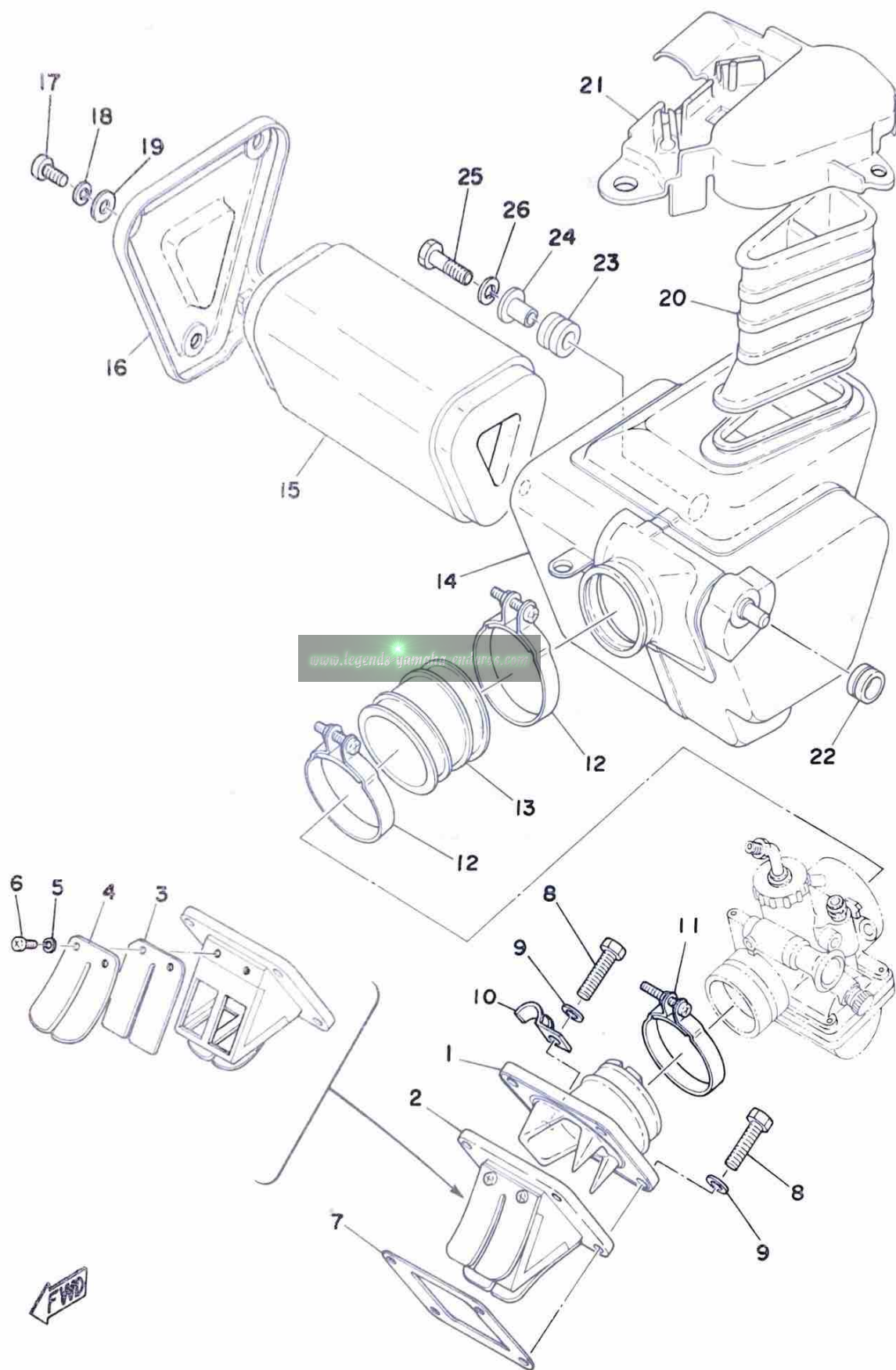
Fig. 9 INTAKE
