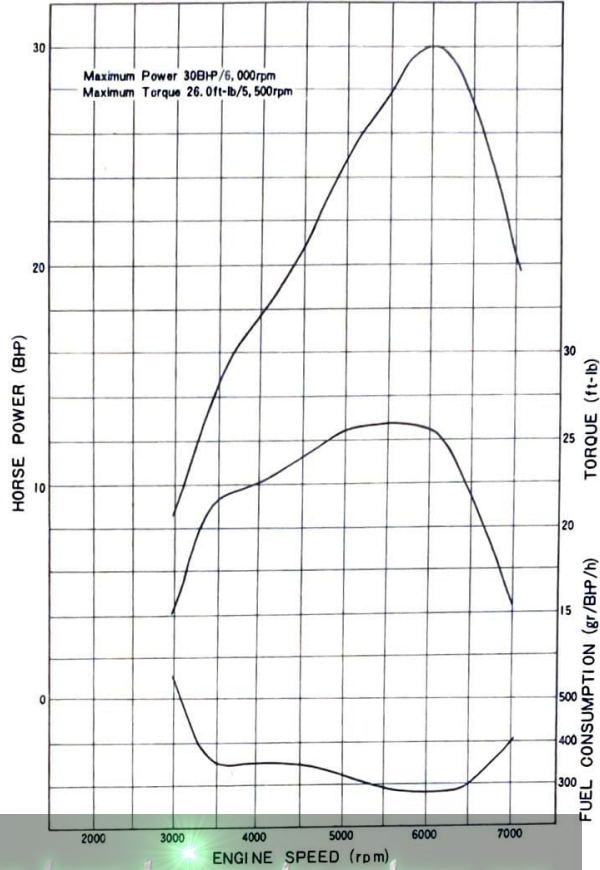
RTI ENGINE PERFORMANCE CURVES
