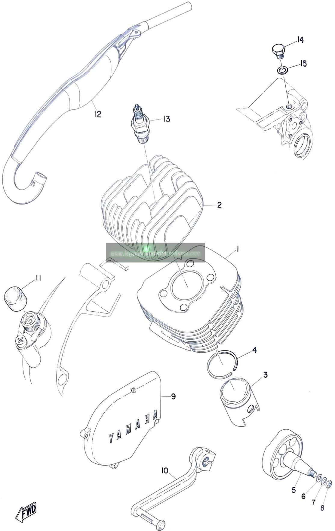
Fig. 1 ENGINE
