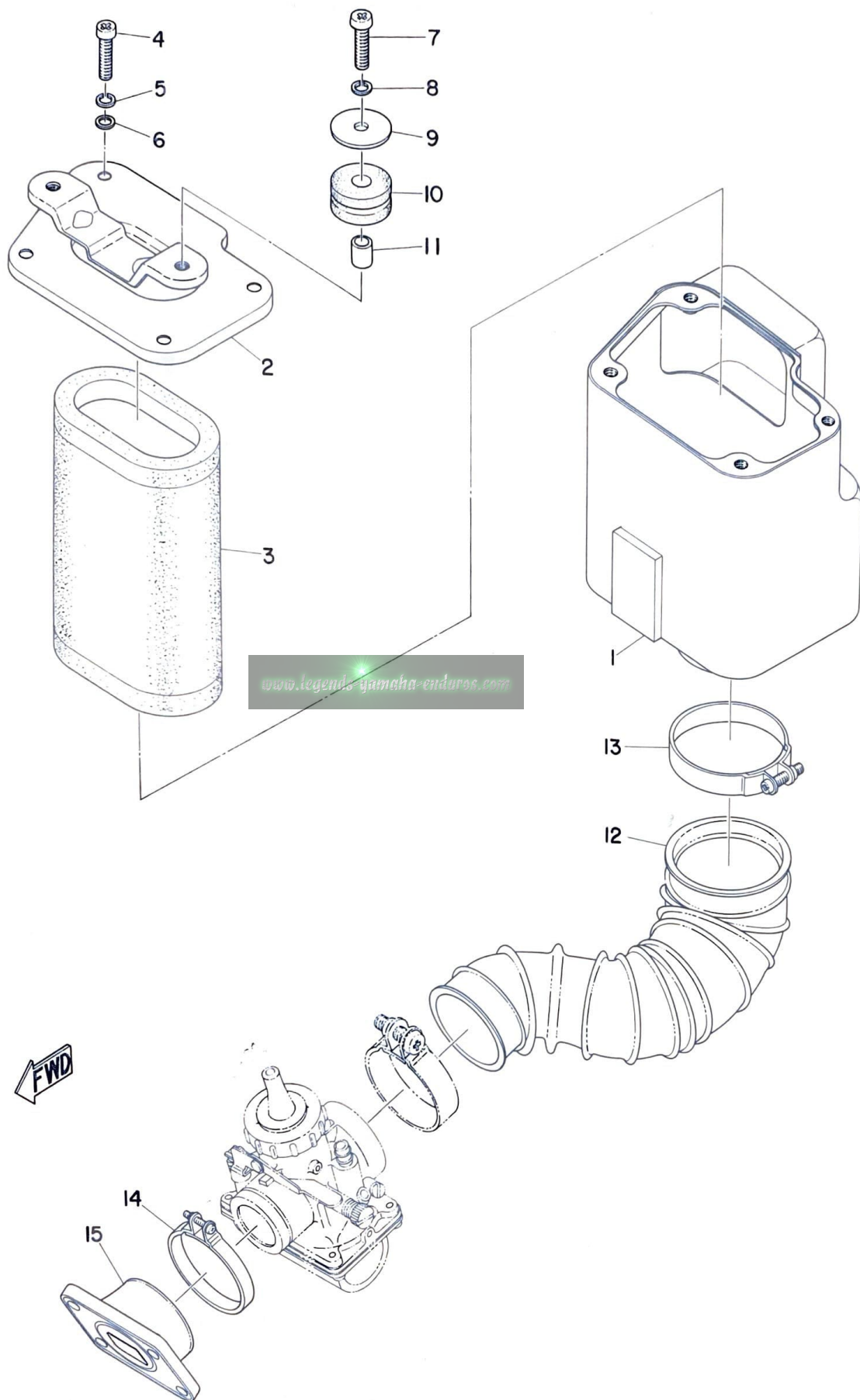
Fig. 3 AIR CLEANER
