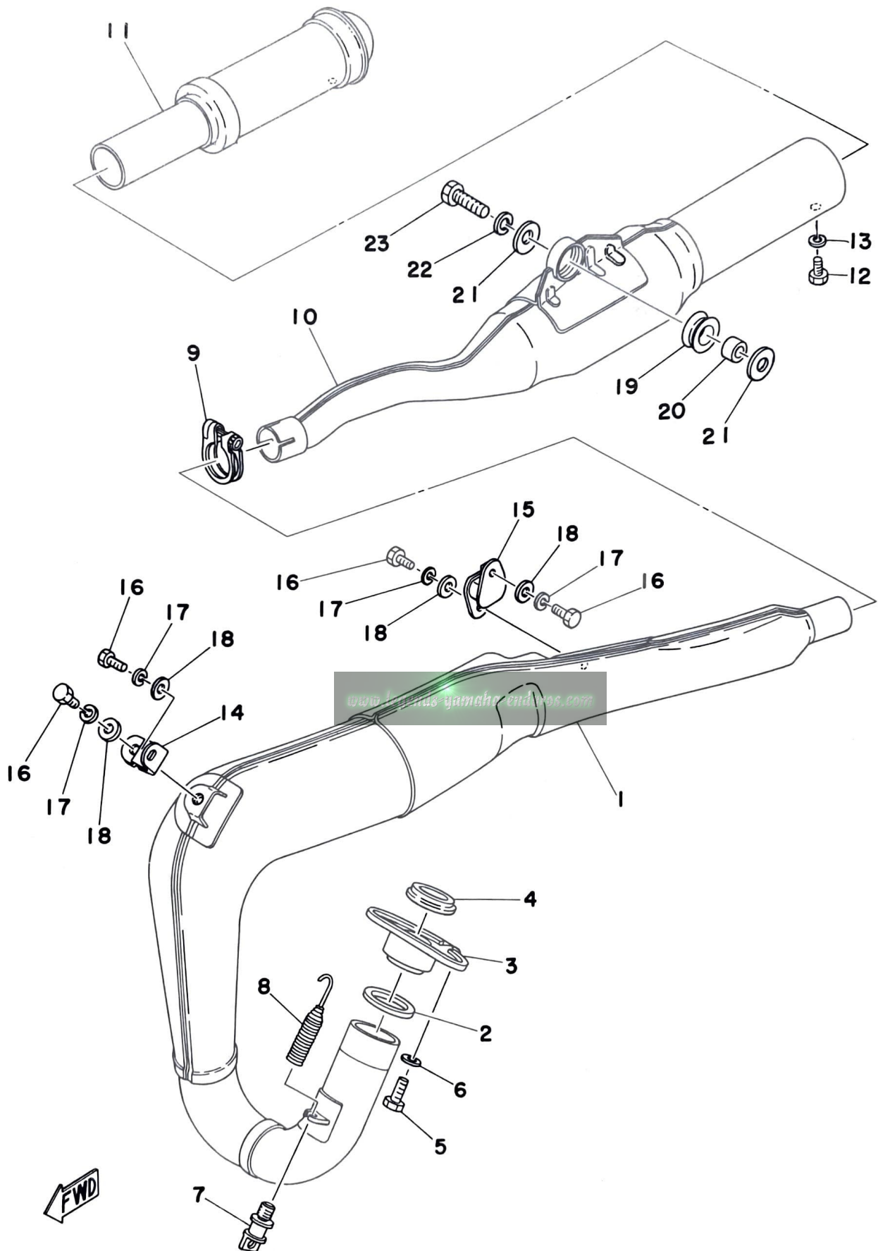
Fig. 11 EXHAUST
