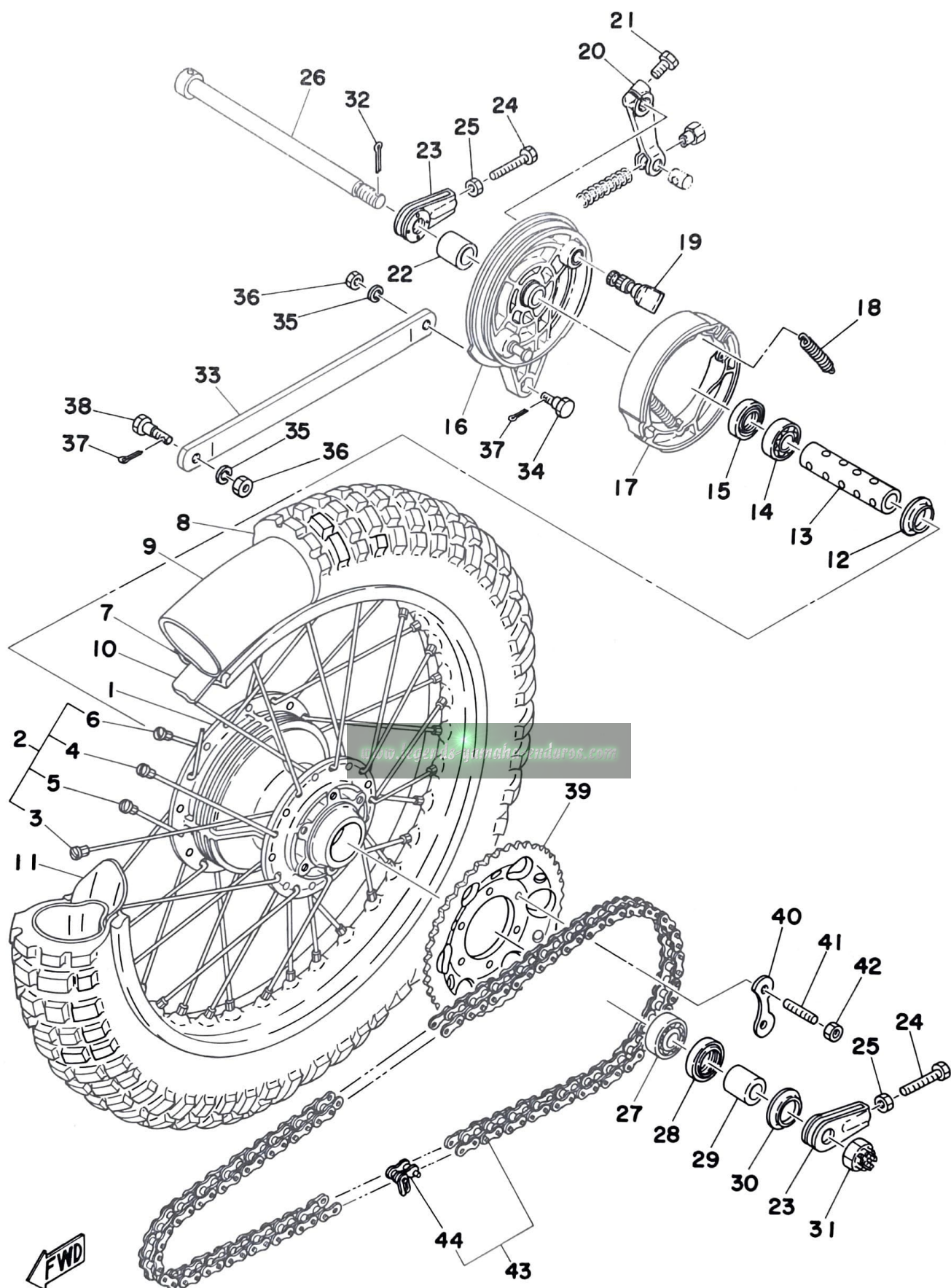
Fig. 23 REAR WHEEL
