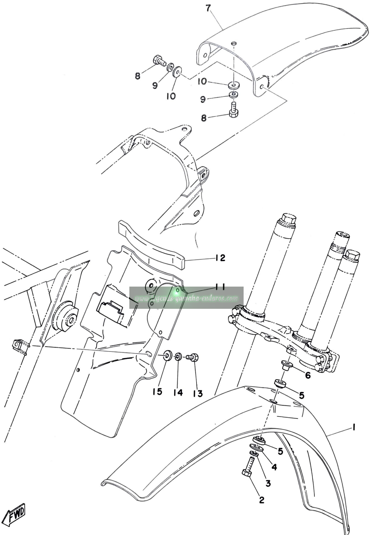
Fig. 16 FRONT FENDER · REAR FENDER
