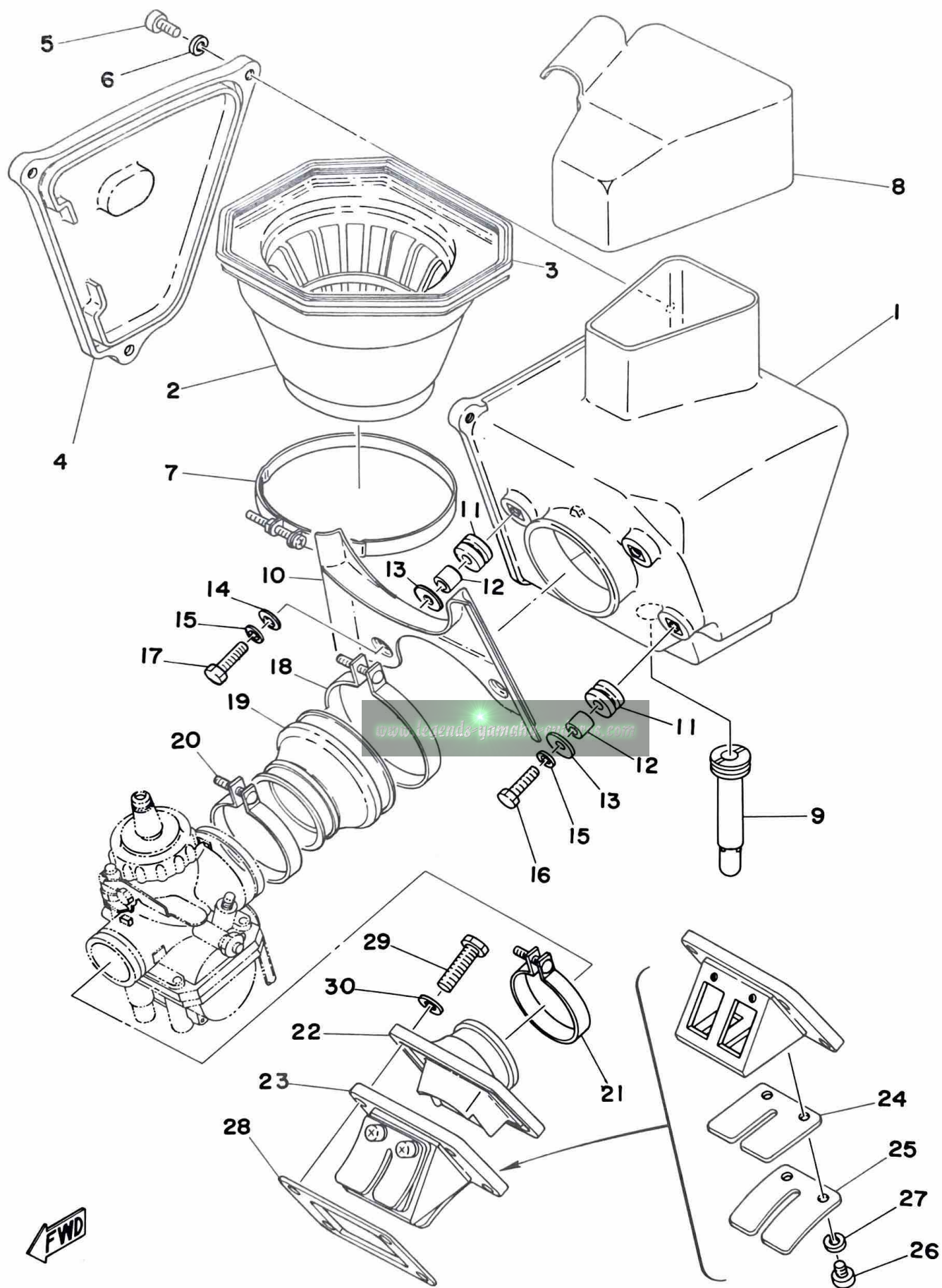
Fig. 9 INTAKE
