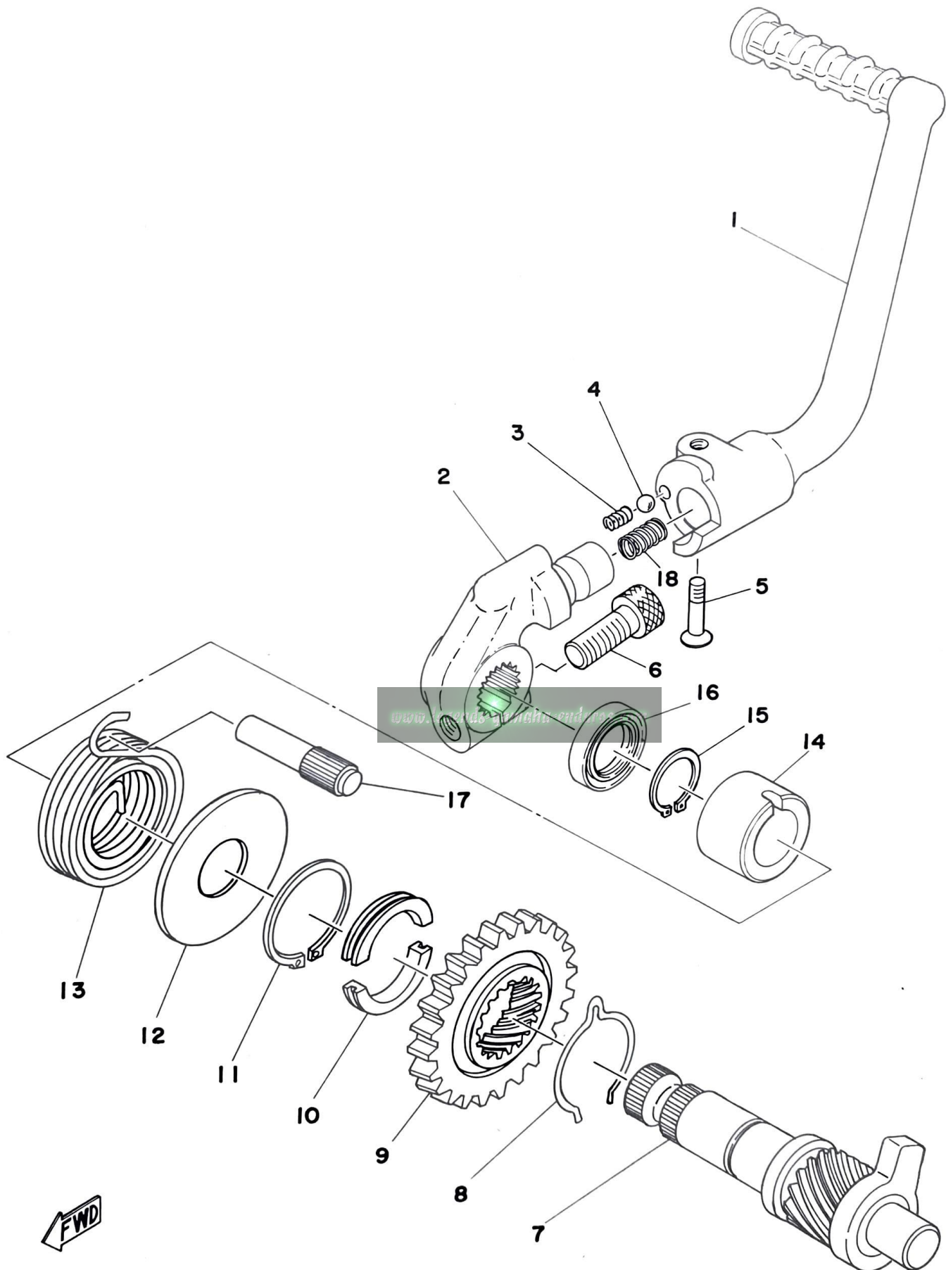
Fig. 8 KICK STARTER
