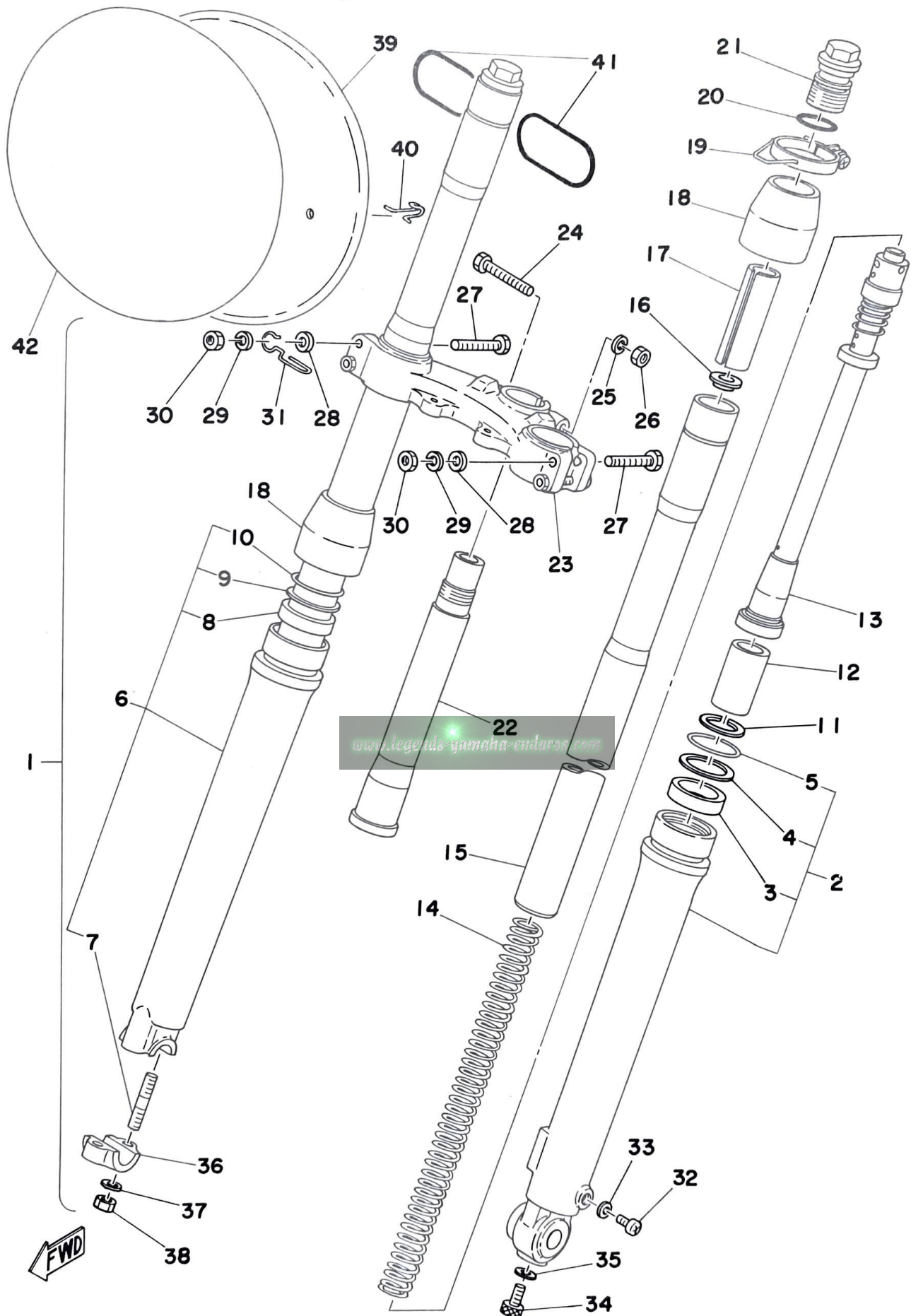
Fig. 17 FRONT FORK
