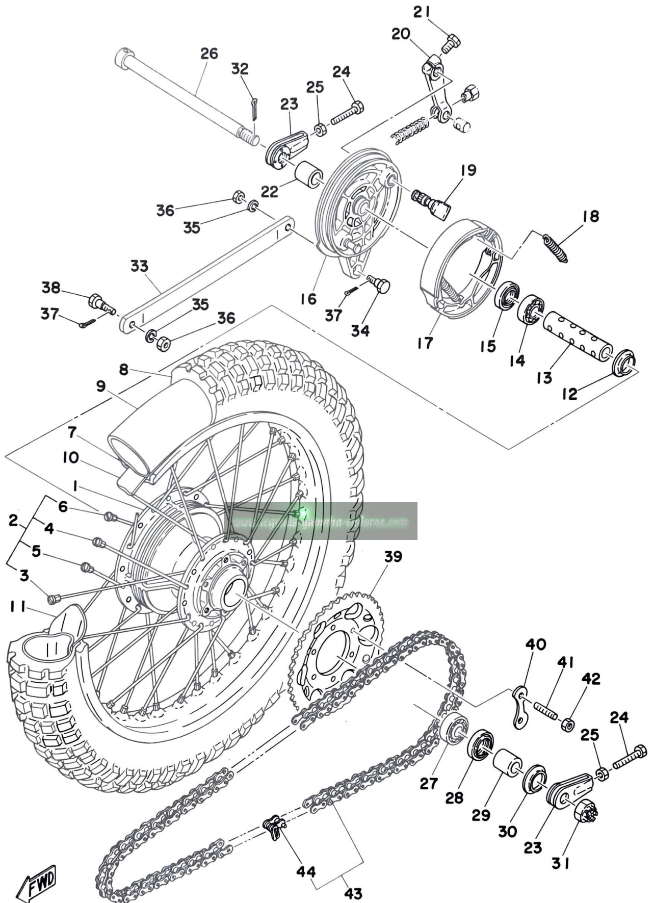
Fig. 23 REAR WHEEL
