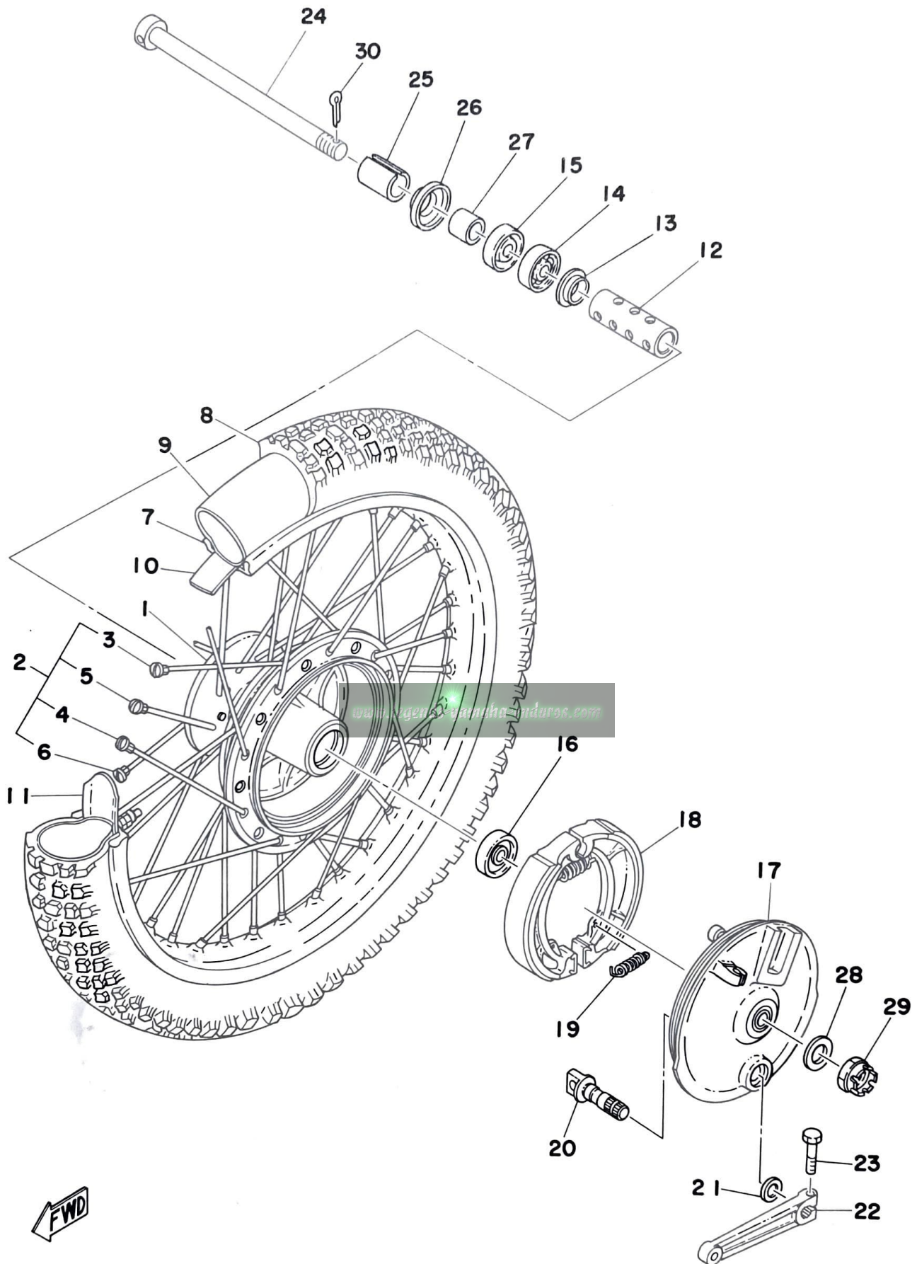
Fig. 22 FRONT WHEEL
