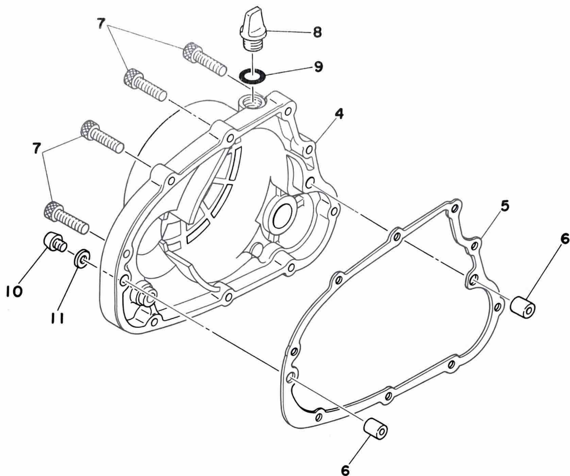
Fig. 2 CRANKCASE COVER
