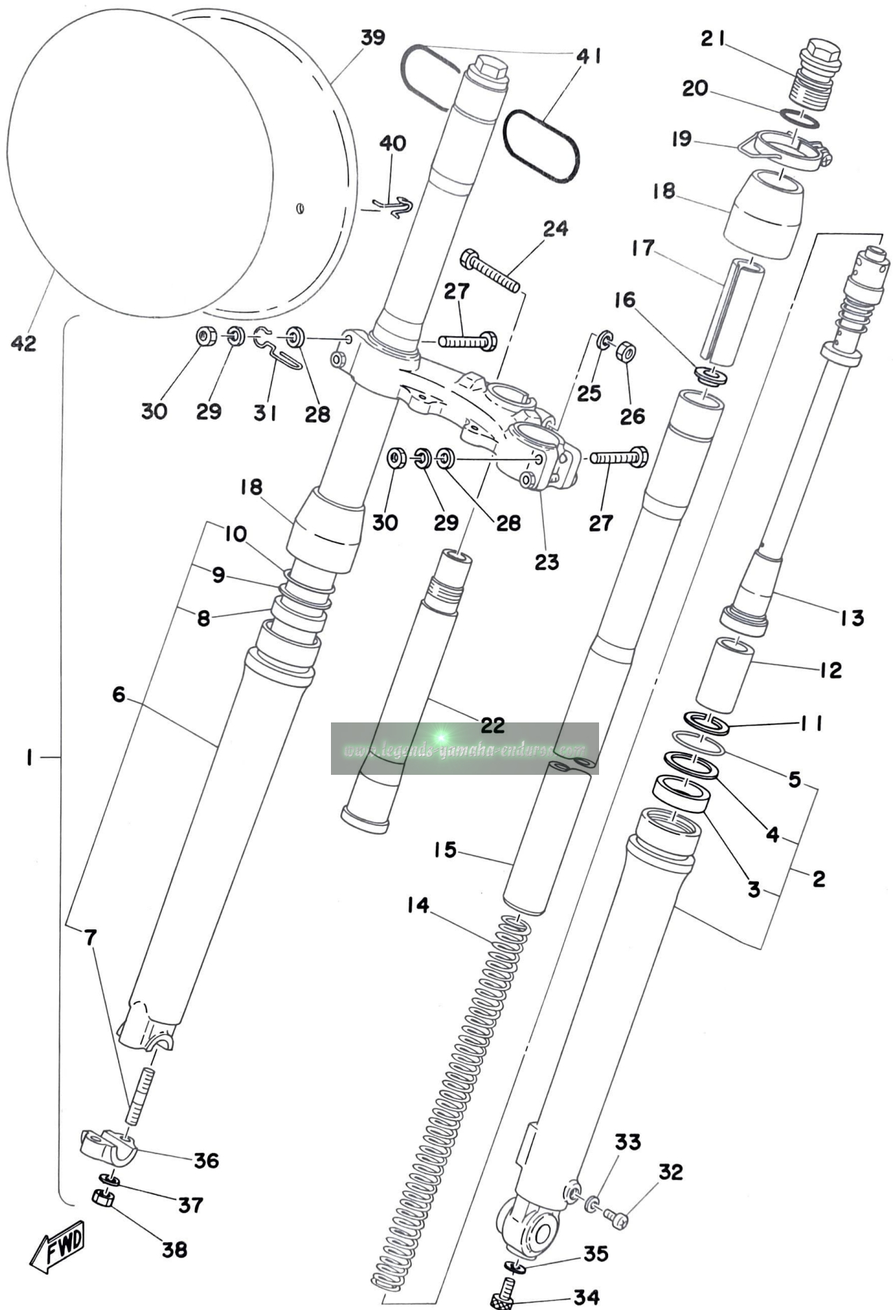
Fig. 17 FRONT FORK
