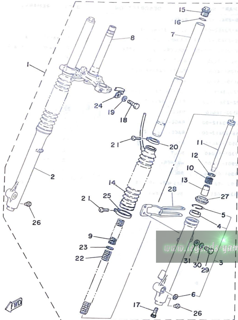
0H1P33TE IS • FIG. 22 FRONT FORK
