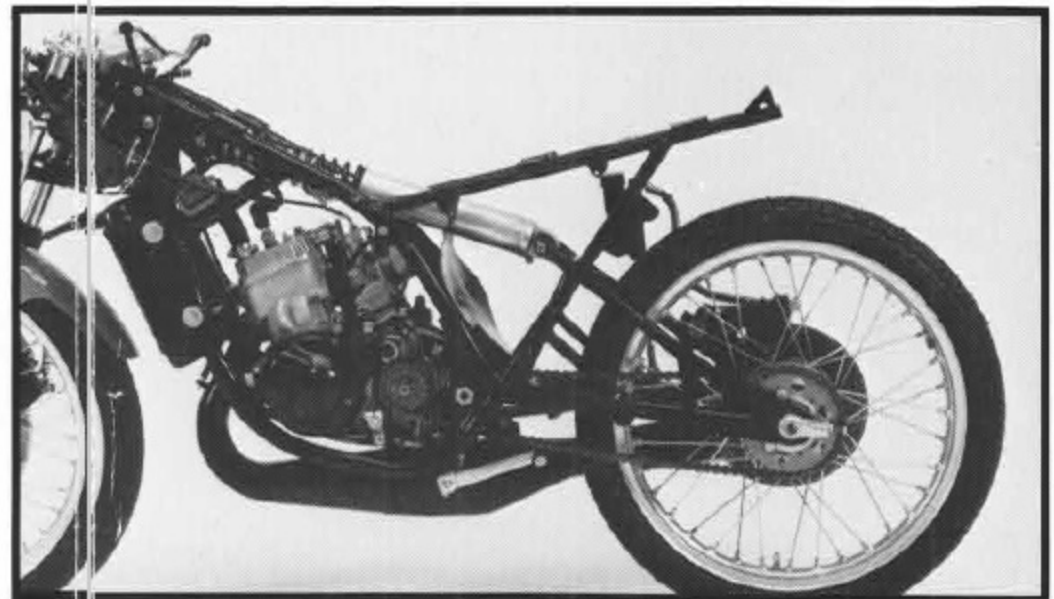
Monocross rear suspension incorporates a large-capacity adjustable damper unit, inert gas, oil, coil spring and bottoming-preventive rubber.
