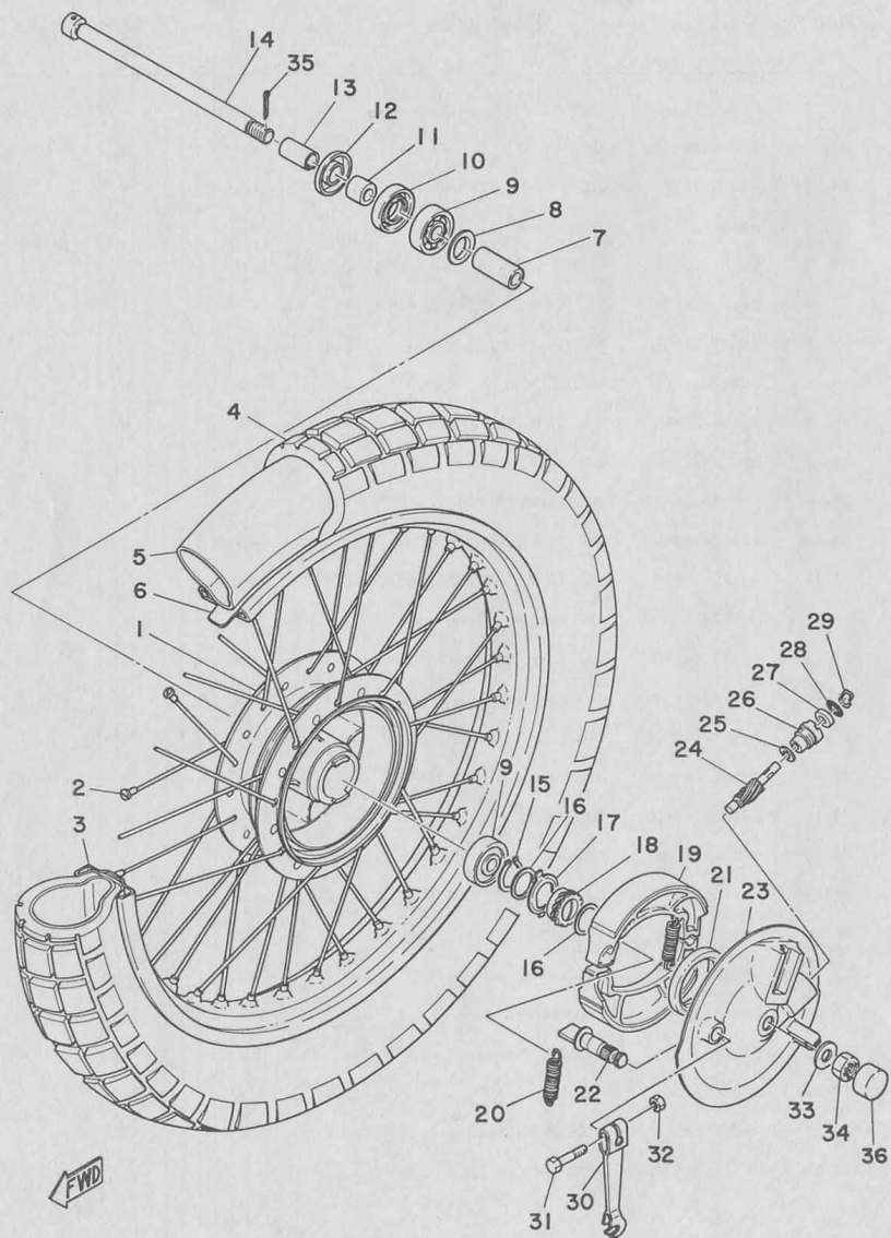
Fig. 25 FRONT WHEEL
