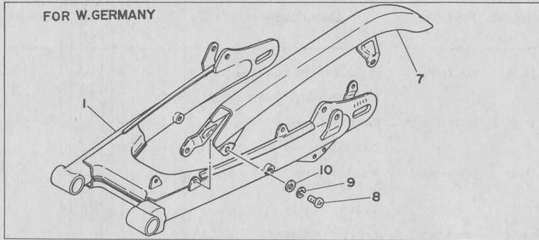
Fig. 16 REAR ARM · REAR CUSHION · CHAIN CASE
