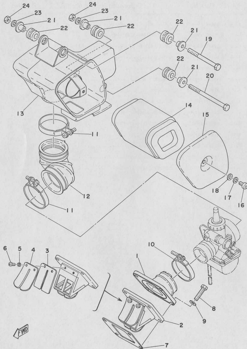
Fig. 10 INTAKE
