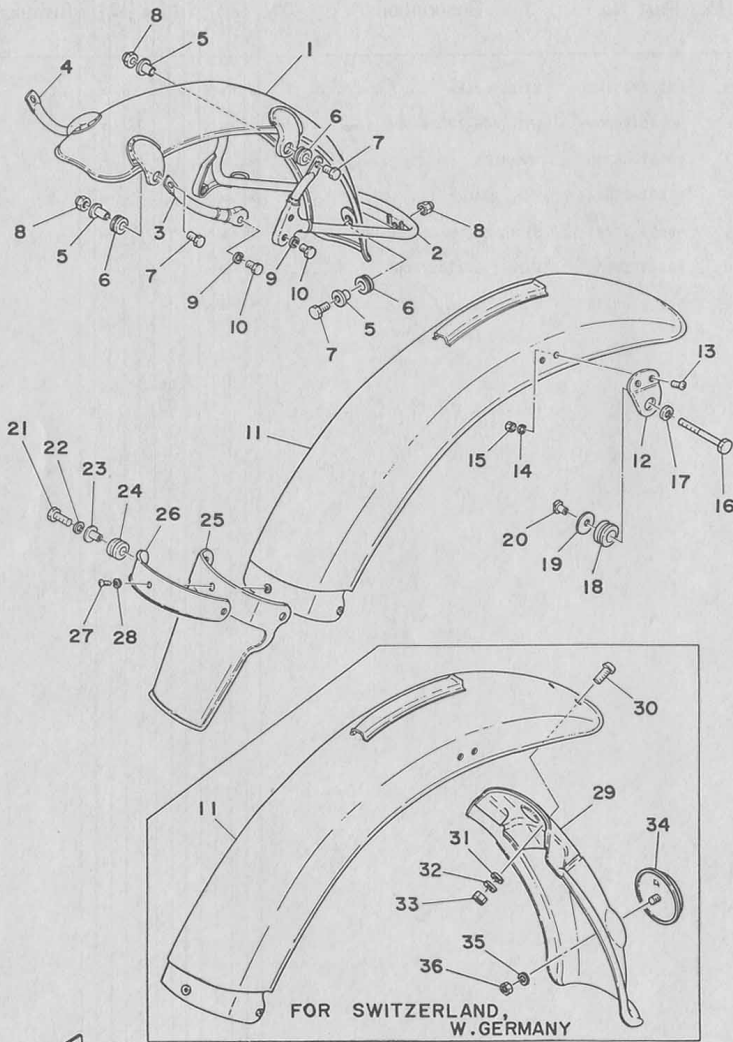
Fig. 18 FRONT FENDER · REAR FENDER
