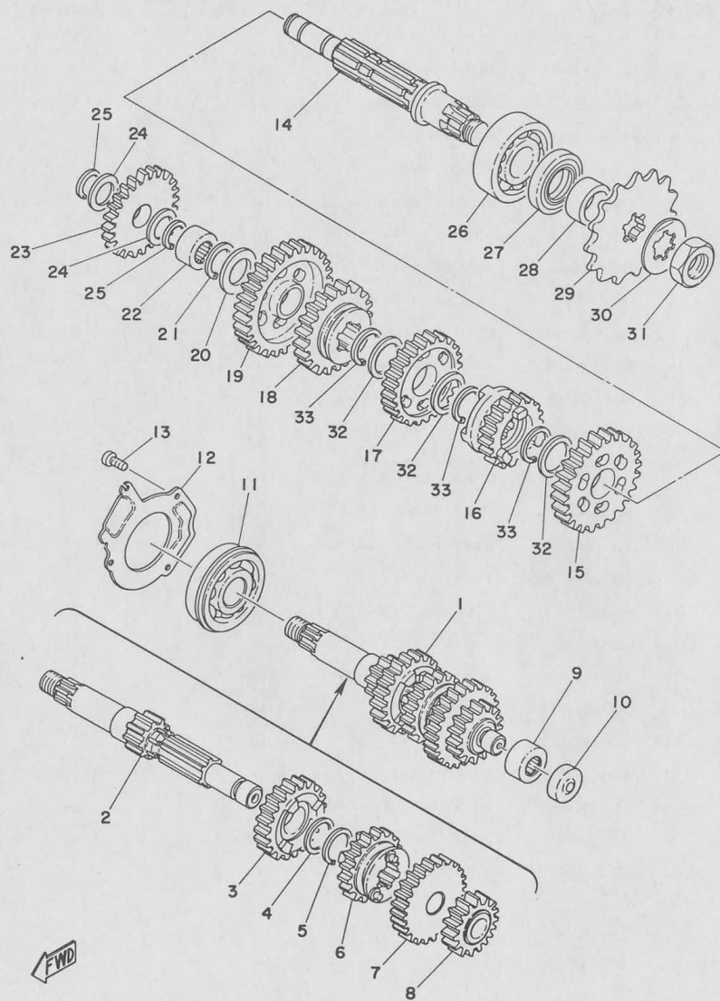
Fig. 5 TRANSMISSION
