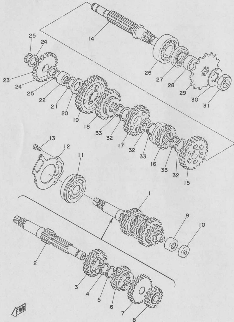
Fig. 5 TRANSMISSION
