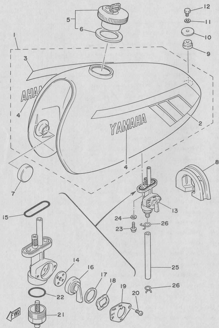
Fig. 22 FUEL TANK
