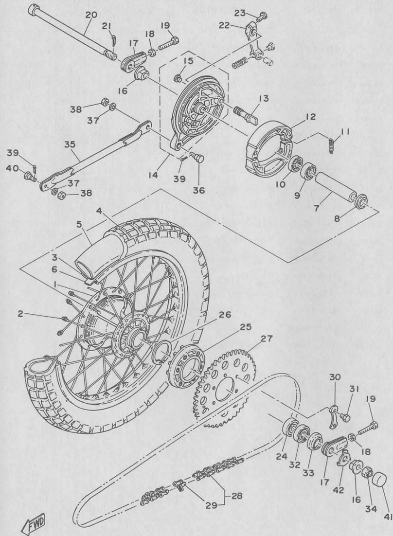
Fig. 26 REAR WHEEL
