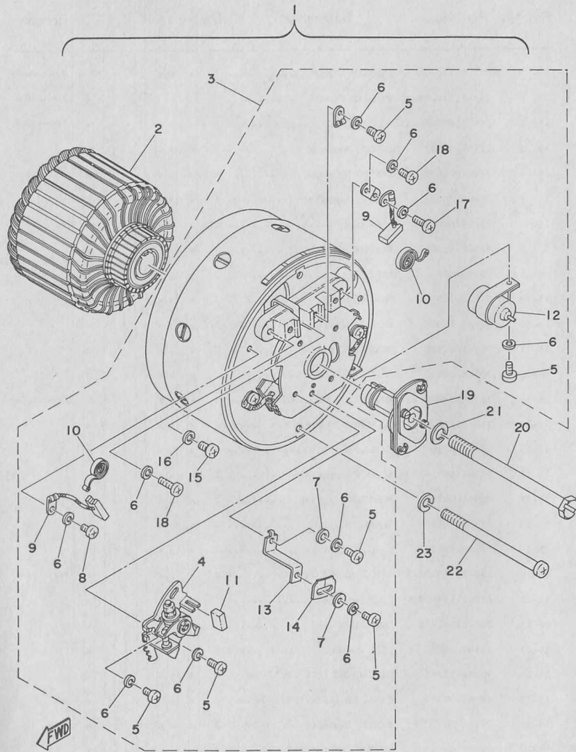
Fig. 14 STARTER GENERATOR
