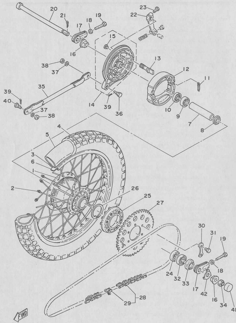
Fig. 26 REAR WHEEL
