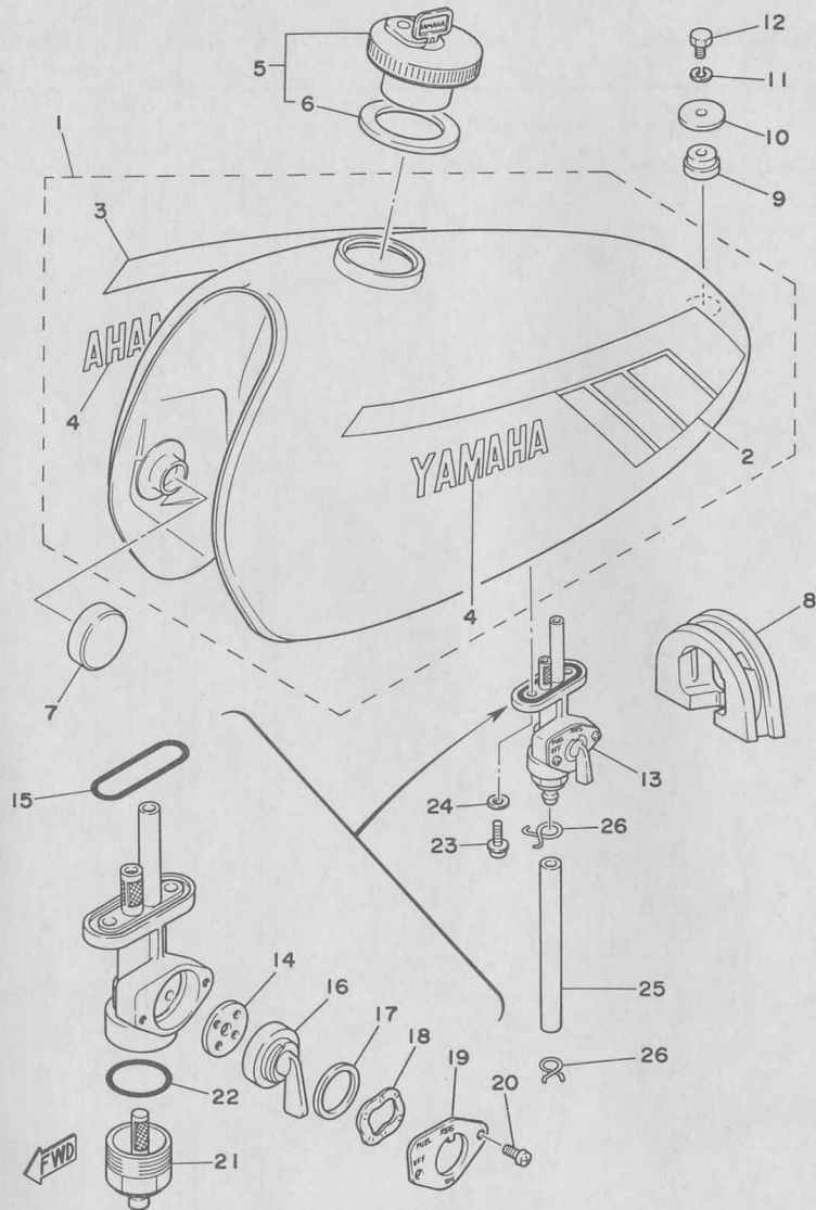
Fig. 22 FUEL TANK
