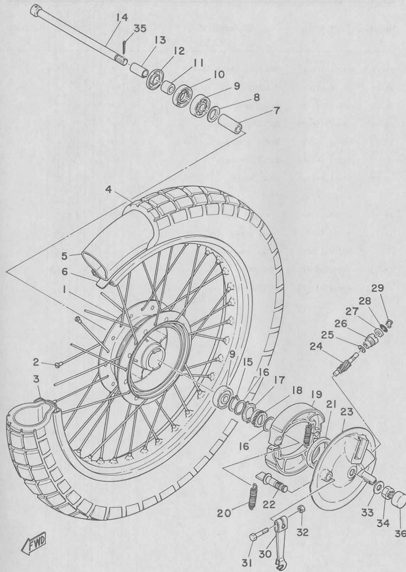
Fig. 25 FRONT WHEEL
