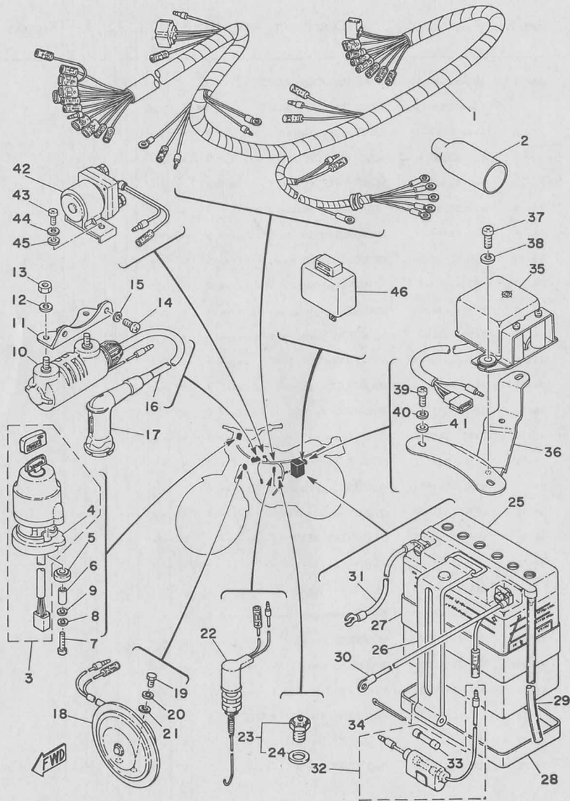
Fig. 34 ELECTRICAL
