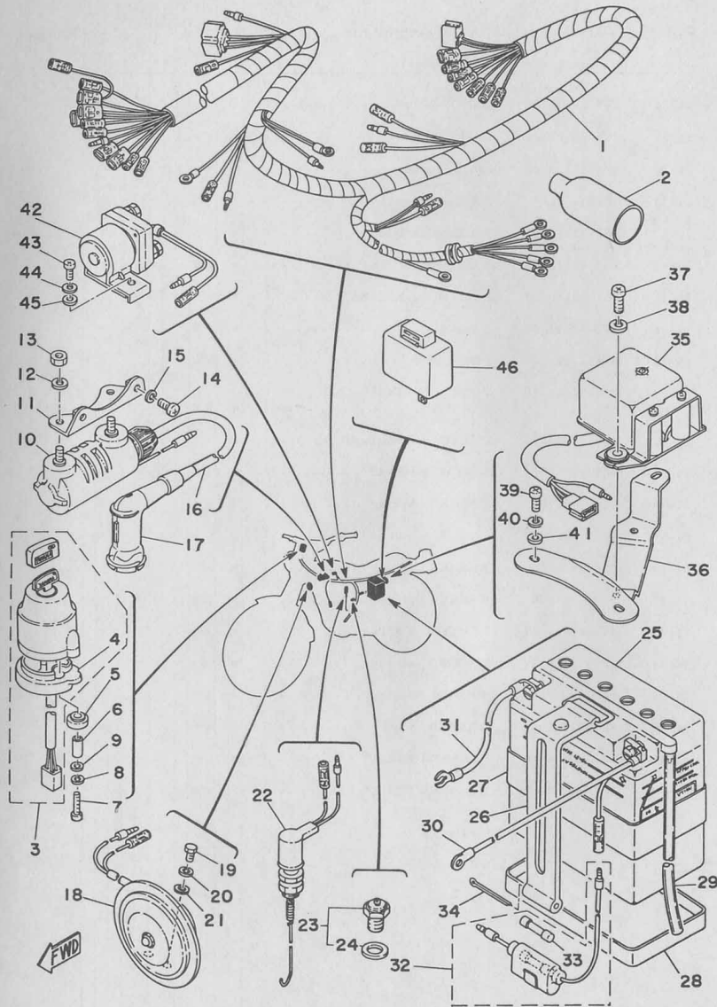
Fig. 34 ELECTRICAL
