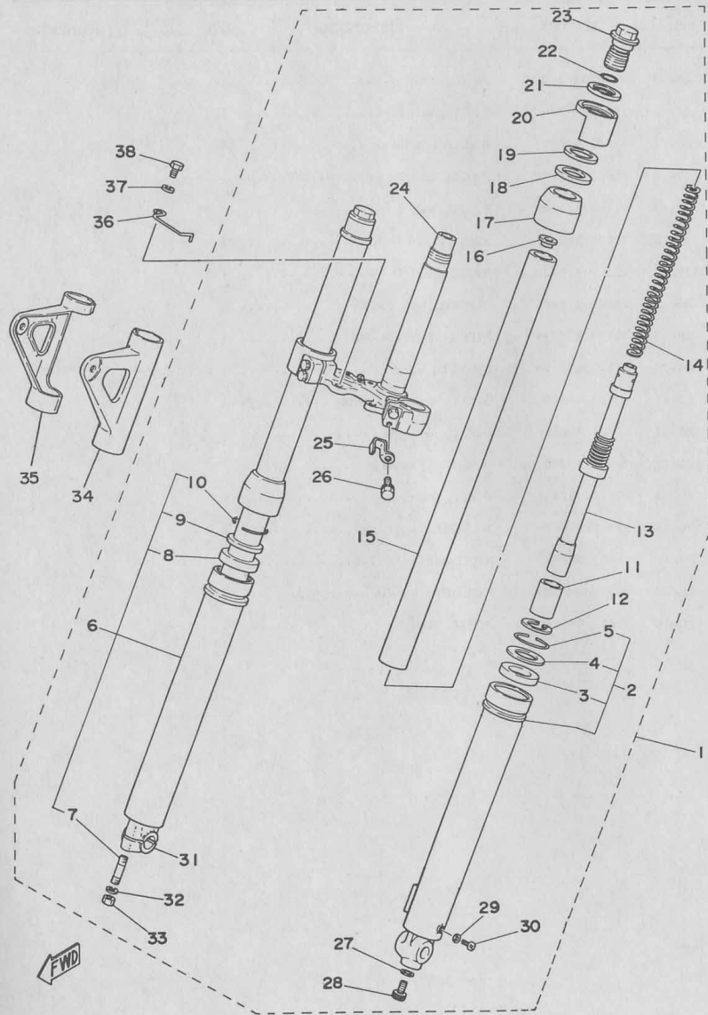
Fig. 19 FRONT FORK
