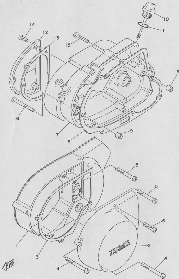
Fig. 2 CRANKCASE COVER
