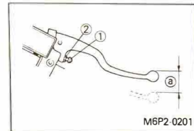
1. Adjuster 2. Locknut a. Free play
