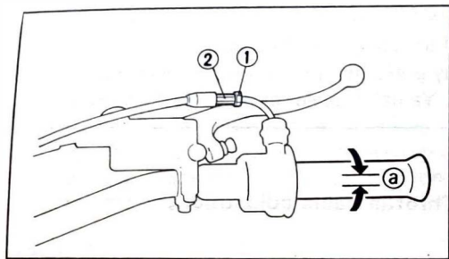
1. Lock nut 2. Adjuster a. 3~5 mm (0.12~0.20 in)
