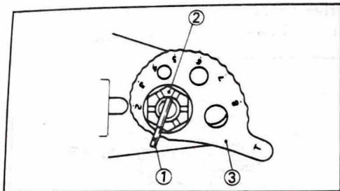
1. Cotter pin 2. Axle nut 3. Chain puller
