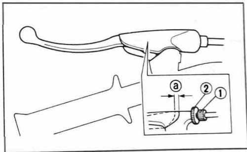
1. Adjuster 2. Lock nut a. 2~3 mm (0.08~0.12 in)
