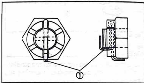
1. Cotter pin
