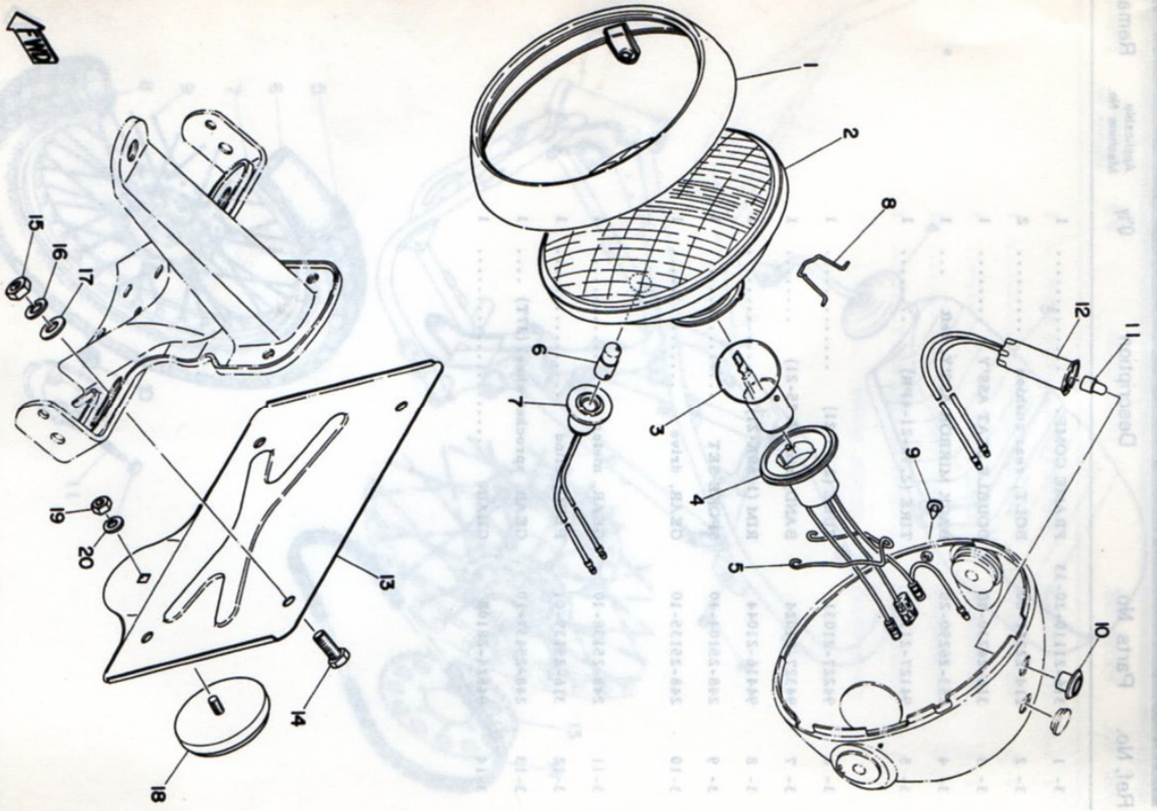
Fig. 4 HEAD LAMP · TAIL LAMP
