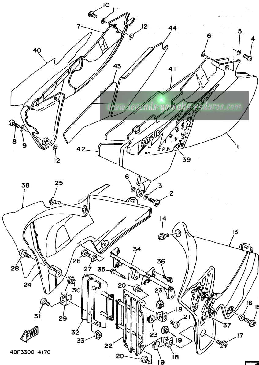
FIG. 17 SIDE COVER
